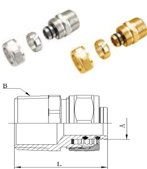
Male straight coupling
