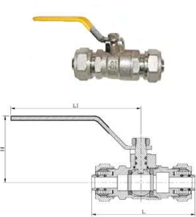
Gas valve EB-NN-0100
