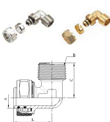
Male elbow
